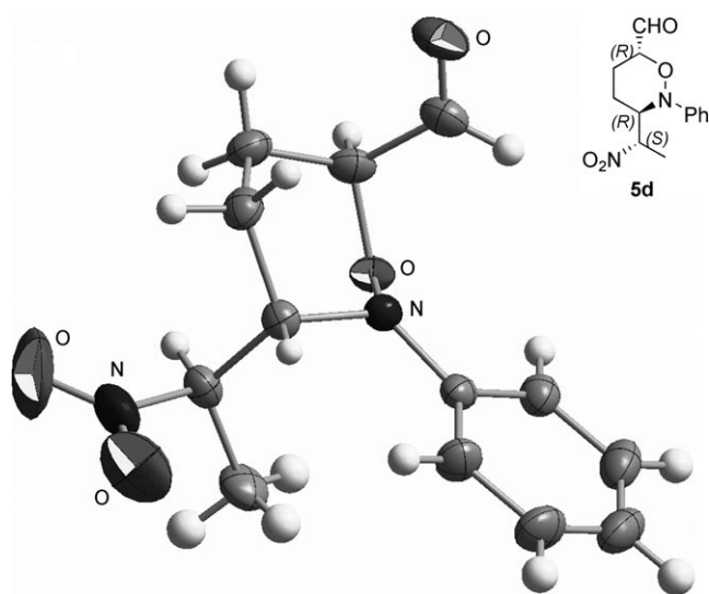
Figure 1. X-ray crystal structure of 5d . [16]
