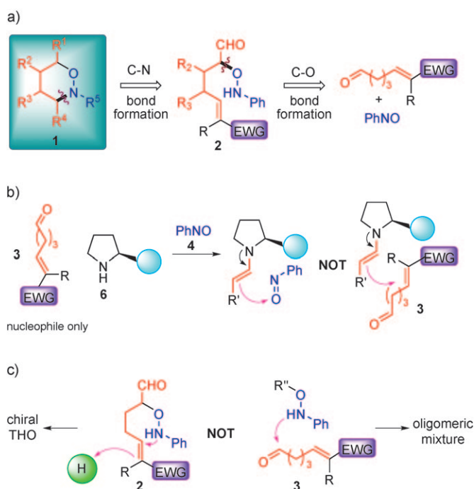
Scheme 1. Proposed synthesis of chiral THO 1 . a) Enantioselective organocatalytic THO synthesis by a C–O/C–N sequence. b) Enamine-catalyzed \alpha -aminoxylation versus Michael addition. c) Aza-Michael addition versus nucleophilic attack on the C=O group and subsequent asymmetric protonation. EWG = electron-withdrawing group.
