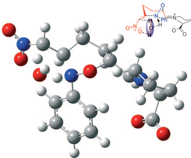
Figure 2. DFT-calculated lowest energy transition state for the aza-Michael addition/protonation in CH 3 CN. [19]
